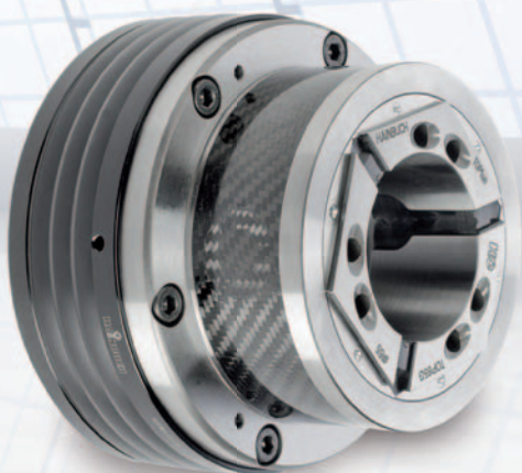
TOPlus CFK Spannfutter
